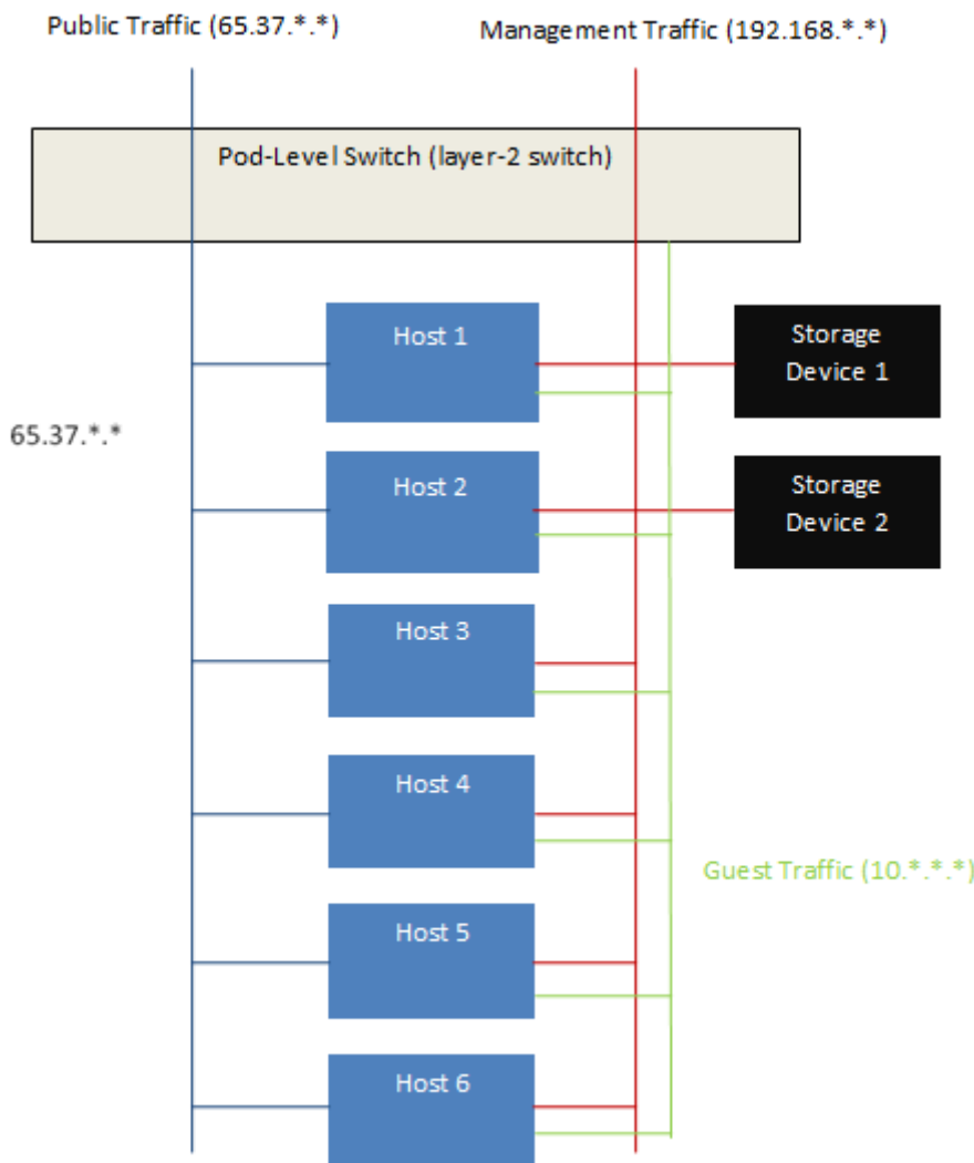
Network Setup within a Single Pod – Logical View
